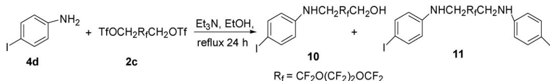
Scheme 6. Reaction of 2c with 4-iodobenzeneamine.
