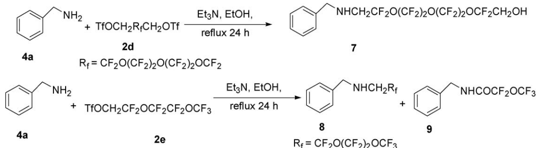
Scheme 4. Reaction of trifluoromethylsulfonate and trifluoromethoxy derivatives with benzylamine.
