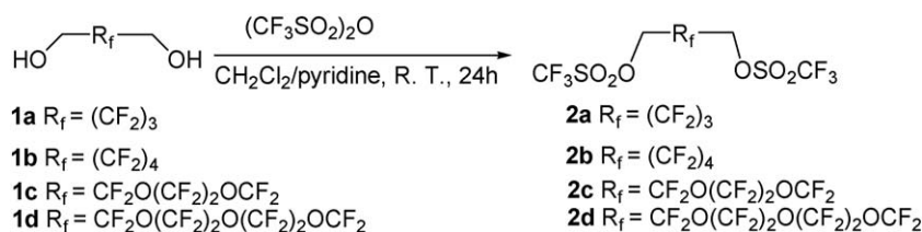
Scheme 1. Syntheses of trifluoromethanesulfonic acid polyfluoroalkyldiyl esters.
