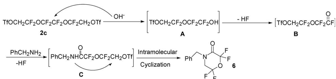
Scheme 5. A plausible reaction mechanism for the formation of 6 .
