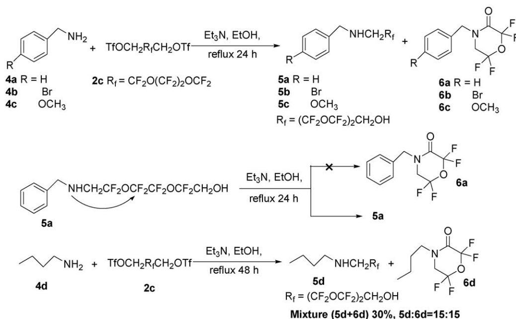
Scheme 3. Synthesis of 2,2,6,6-tetrafluoro-4-phenylmethylmorpholin-3-one.
